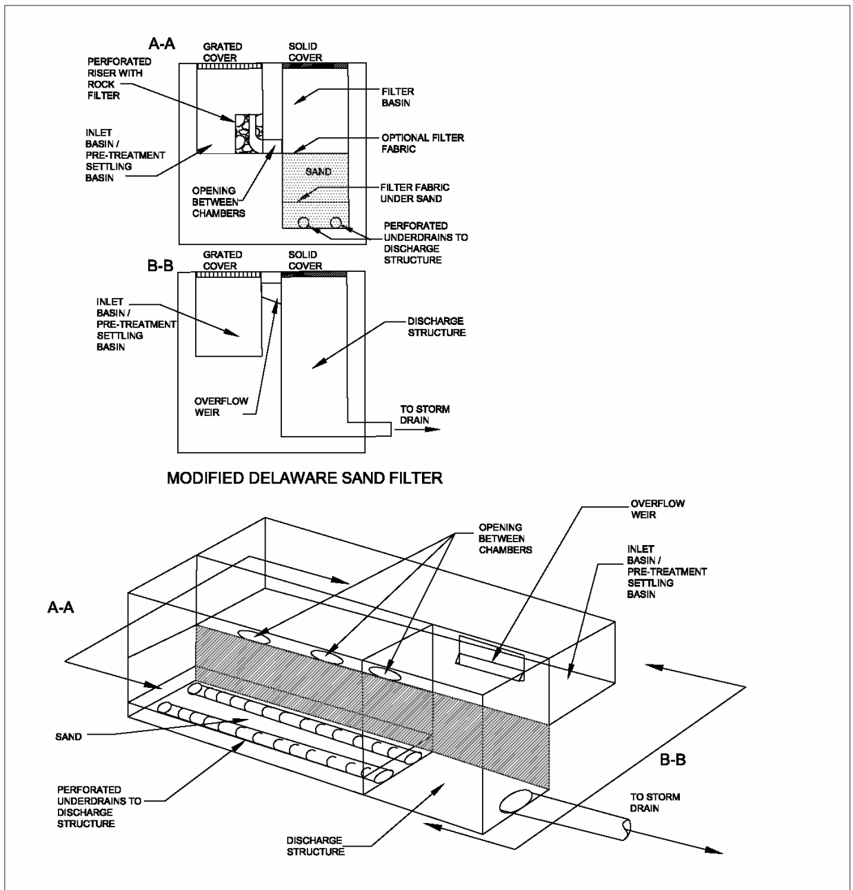
Figure 6-17. Cut Away Profile Views, System A Filter
