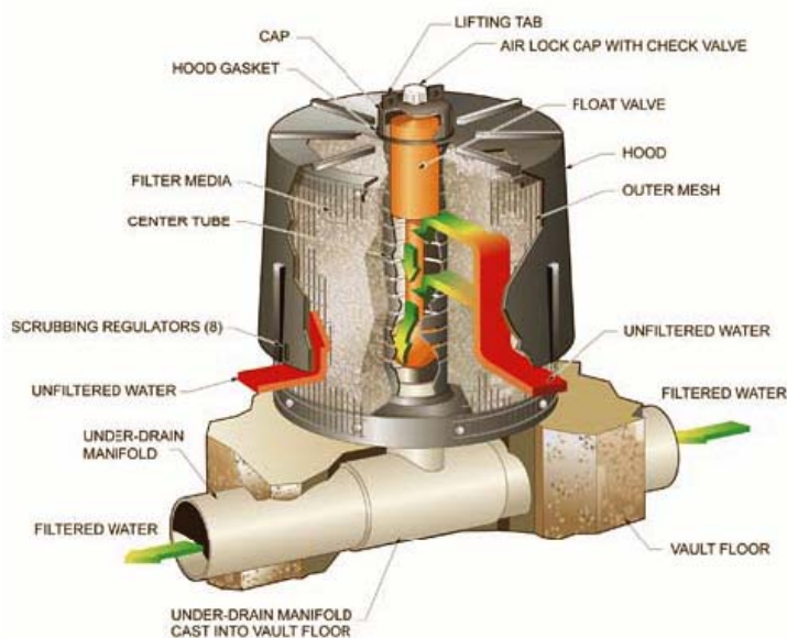
Figure 6-16. System C Filter Cartridge, Typically Used as Part of Treatment Train.
