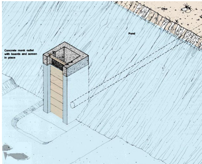
Figure 3-3. Wetland outlet riser and pipe
