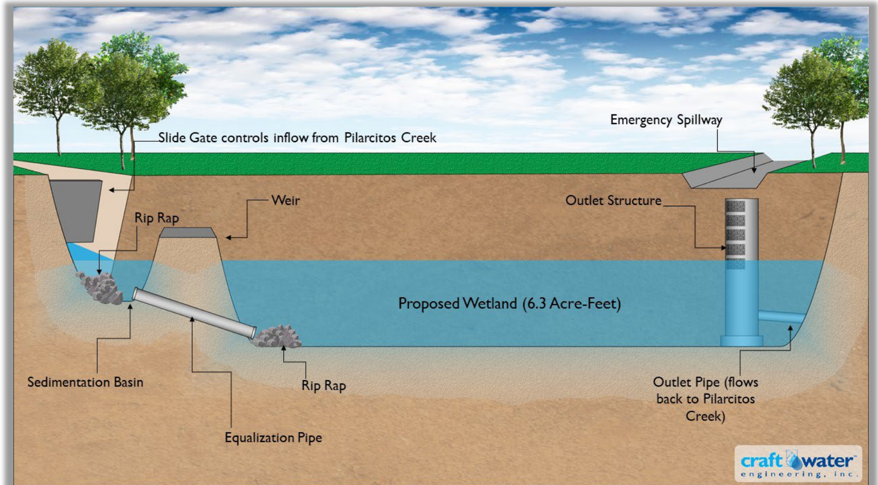
Typical Section
