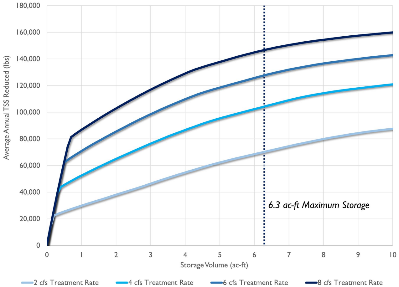
Figure 2-7. Project storage volume vs pollutant reduction for a BMP with a 50 cfs diversion rate at the site.
