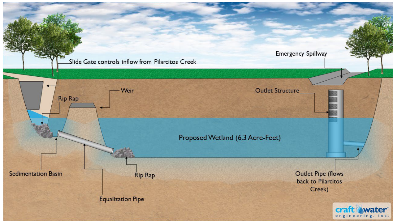
Figure 3-2. Half Moon Bay BMP Preliminary Concept Profile
