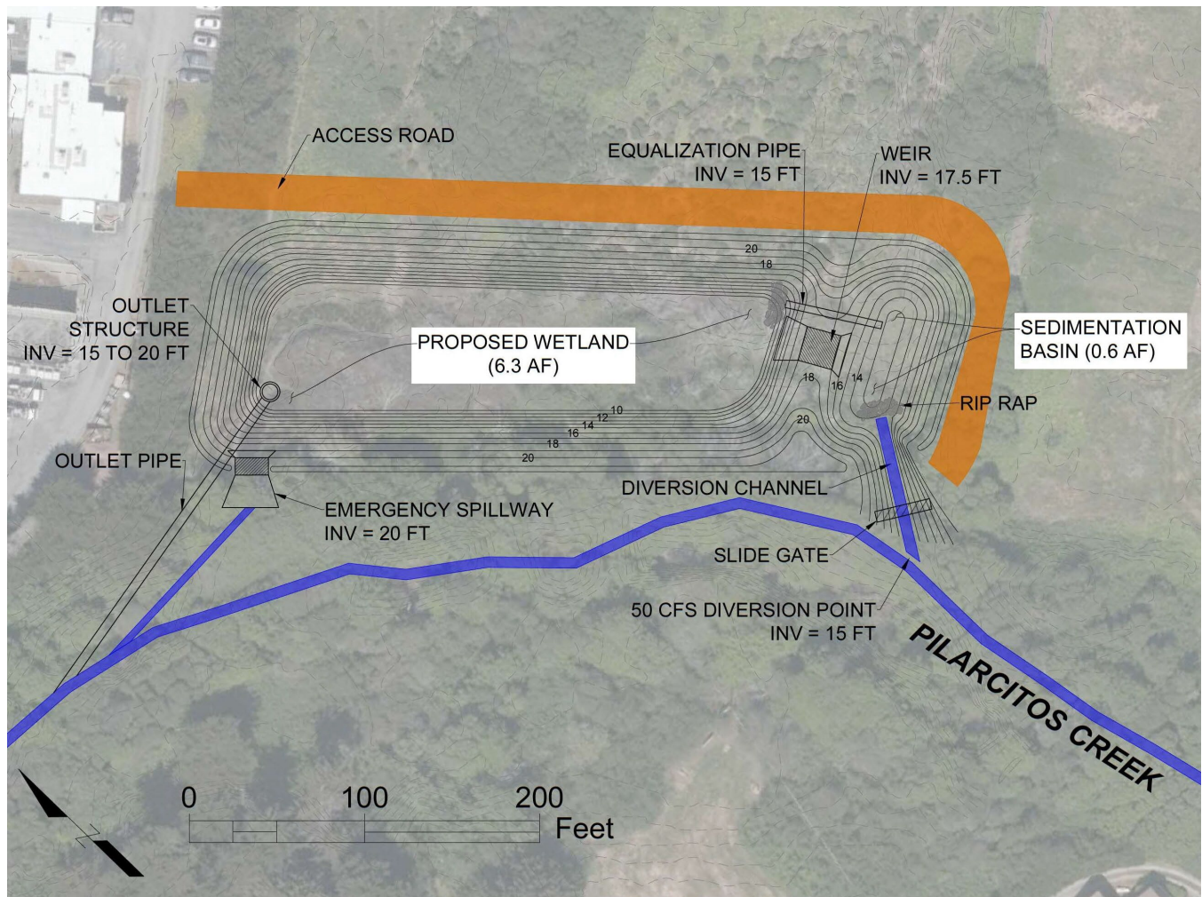
Figure 3-1. Half Moon Bay BMP Layout
